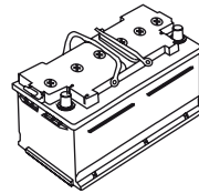
L5B + - 353x175x175 58803
